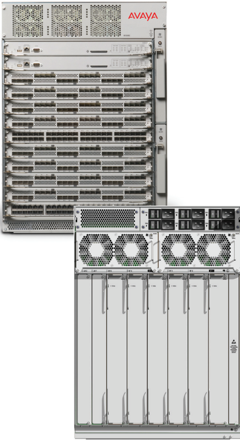
Virtual Services Platform 9000 (front & rear views)
